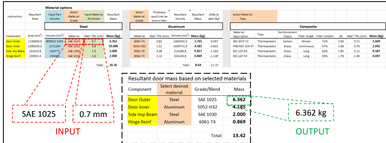
Figure 8: Weight Approximation Model, Steel Door Outer (4 components)
