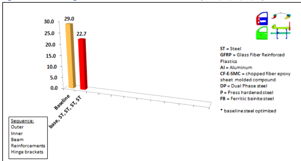
Figure 13: Door Weight from 5 Parts Based on Material (base,ST,ST,ST,ST)
