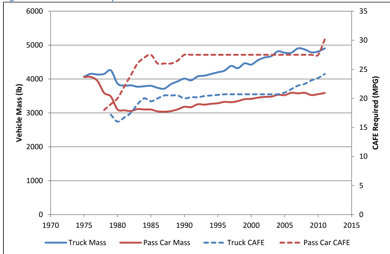
Figure 3: Vehicle Mass in Response to CAFE
