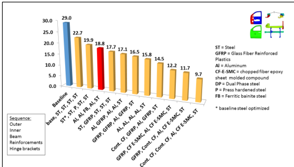
Figure 43: Door Weight from 5 Parts Based on Material (Cont. CF, Cont. CF, AI, CF E-SMC, ST)
