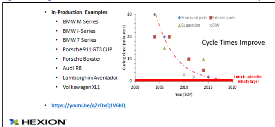
Figure 34: High-Pressure RTM/LCM Process' Continued Reduction in Cycle Times
