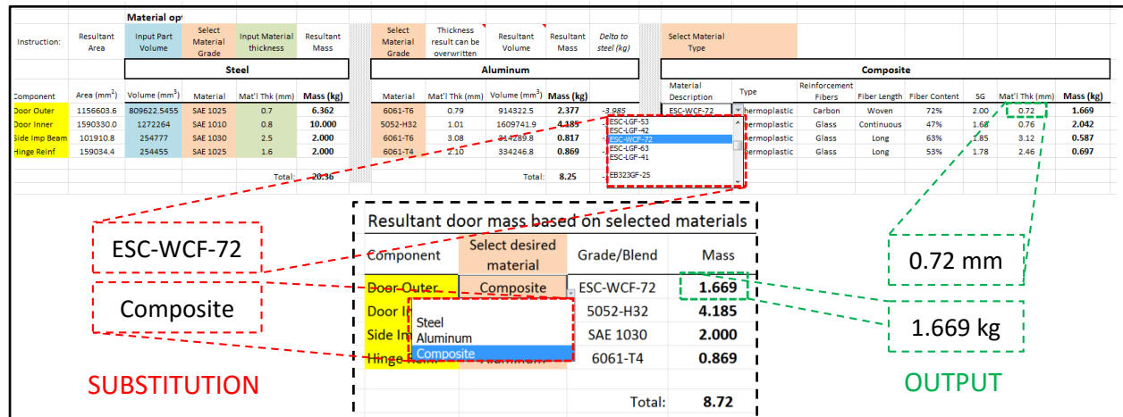
Figure 10: Weight Approximation Model, Composite Door Outer (4 components)
